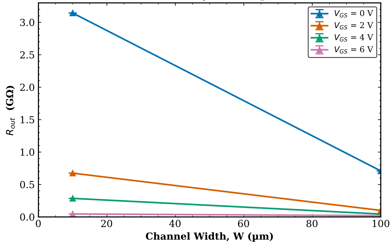
TFT3 Transistor 2 R_{out} vs W | L = 80\text{ }\mu\text{m}
